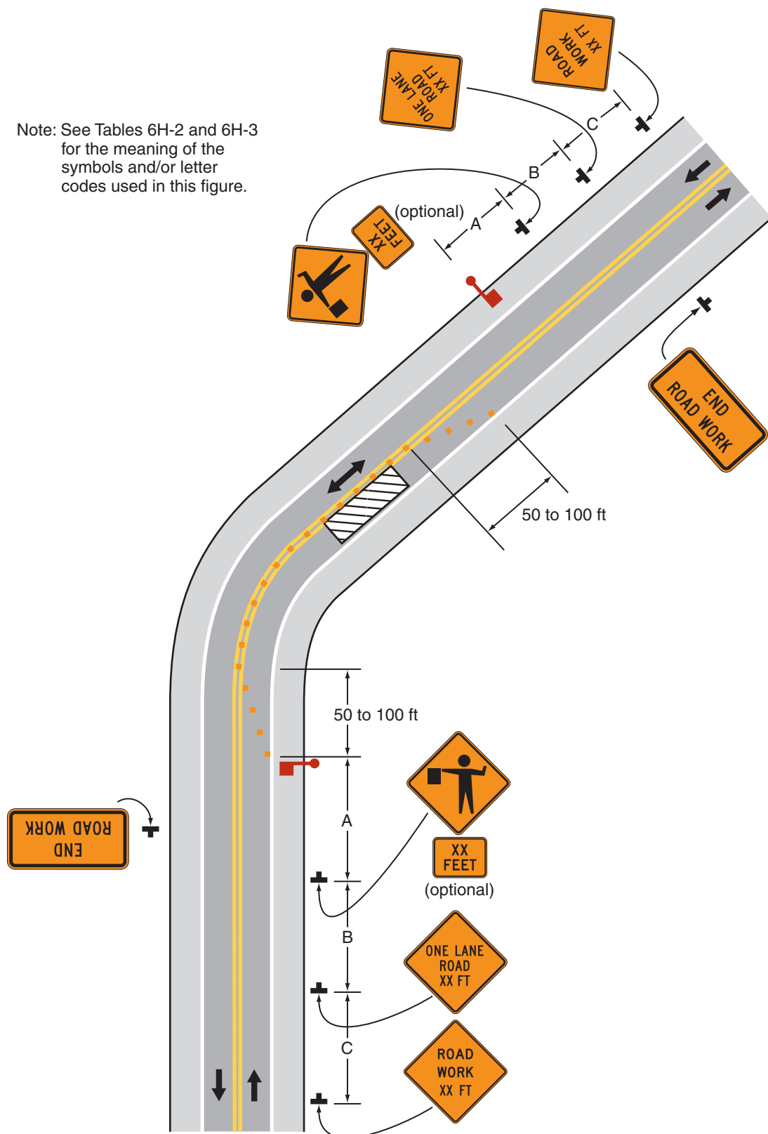
Typical Application 10
