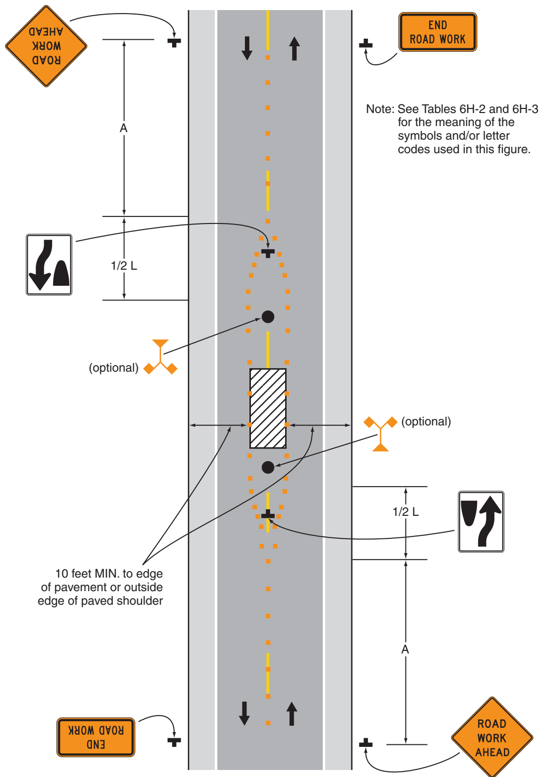
Typical Application 15
